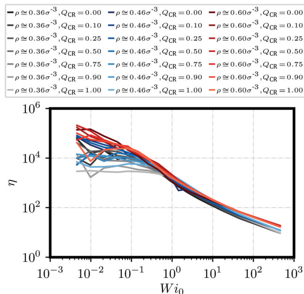
Fig. 3 Polymeric viscosity \eta against Weissenberg number Wi_0 for a variety of different monomer densities \rho and chain monomer fractions Q_{CR} .
