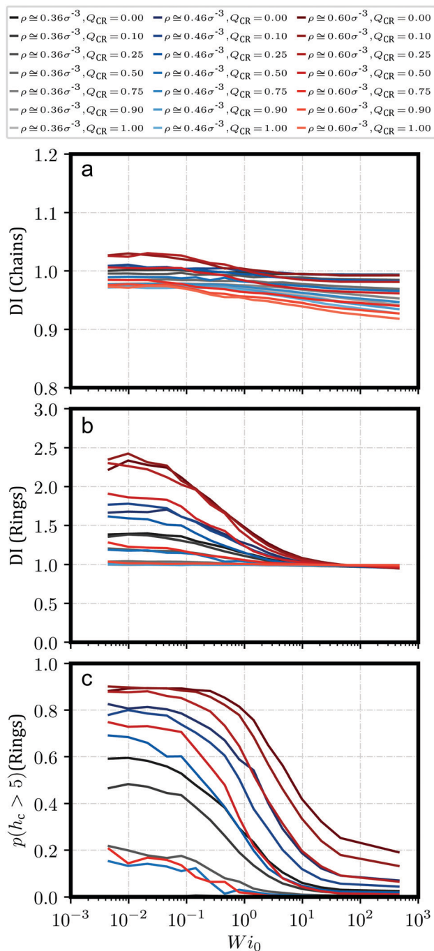
Fig. 2 Quantitative indicators for clustering against Weissenberg number Wi_0 for a variety of different monomer densities \rho and chain monomer fractions Q_{CR} . (a) dispersion index DI, only chains. (b) dispersion index DI, only rings. Values of DI > 1 indicate clustering. (c) probability p(h_c > 5) for a ring to belong to a stack with more than 5 members. Higher probabilities indicate clustering.
