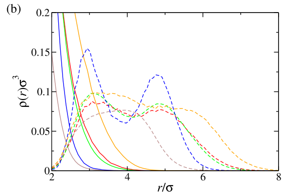
FIG. 12. Radial density profiles for all core and shell monomers with respect to the center of mass of the cluster in BCC crystals for various combinations of average cluster size and density. The solid curves and dashed curves correspond to profiles of core and shell monomers, respectively.
