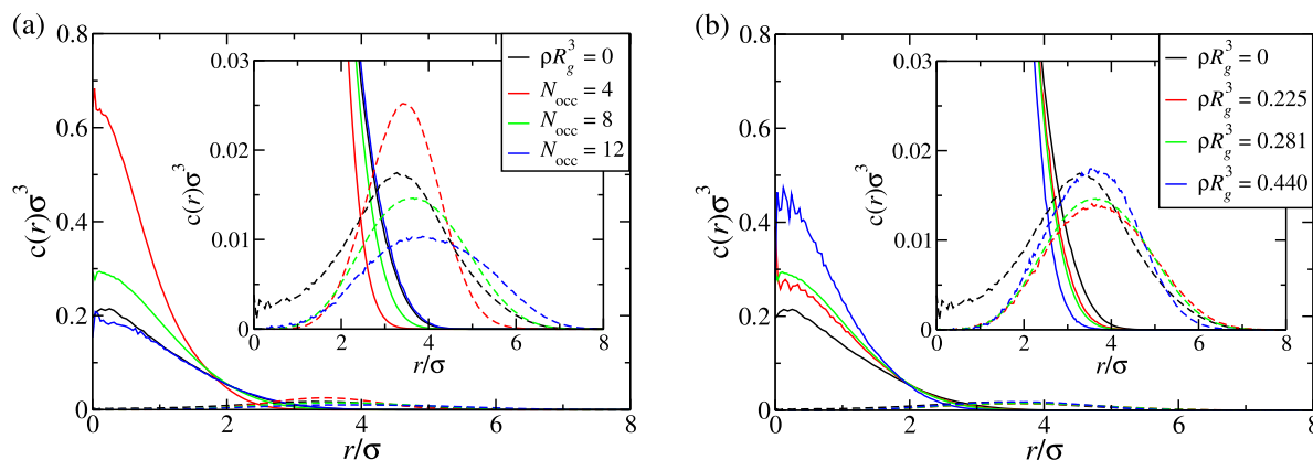
FIG. 9. Single-dendrimer monomer-density profiles \rho(r) with respect to the Model II-dendrimer center of mass in FCC cluster crystals for (a) fixed density \rho R_g^3 = 0.281 and (b) fixed cluster size N_{\text{occ}} = 8 . Solid lines correspond to the core monomers, dashed curves to the shell monomers. Insets are enlargements focusing on the shell monomer profiles. For comparison, the density profiles as found for an isolated dendrimer are shown in black.
