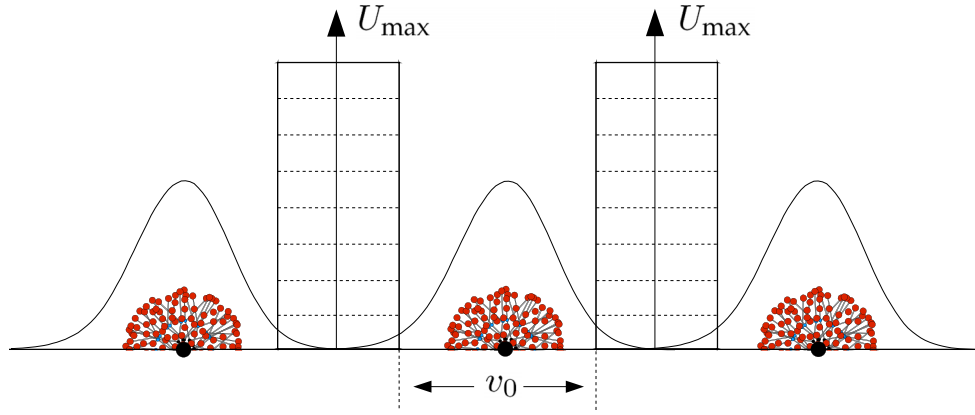
FIG. 13. One-dimensional, schematic representation of the confining potential used in the free energy calculations for cluster crystals. The solid curves represent the density distributions around the lattice sites (black circles). The quantity U_{\max} is the barrier height, see Eq. (13), whereas v_0 indicates the volume left between neighboring barriers in which the particle is free of external influences.
