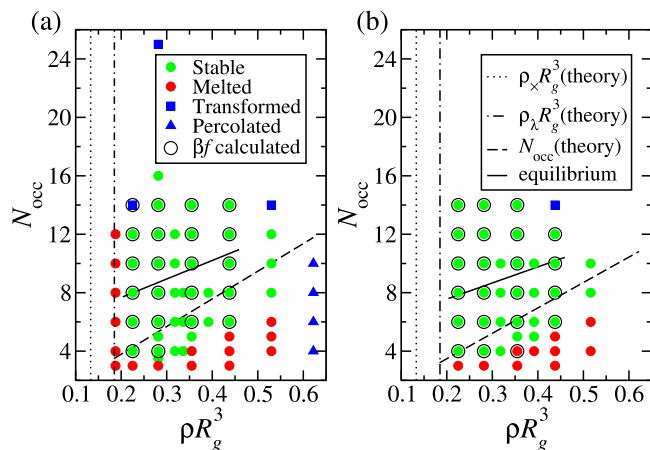
FIG. 7. Mechanical stability diagrams for (a) BCC and (b) FCC crystals for Model II. Stable systems are marked in green, unstable in red or blue. Systems for which the free energy was computed are marked with a black circle. The dotted, dotted-dashed, and dashed lines represent the theoretically predicted freezing densities, Kirkwood instability, and cluster occupancies, respectively. The solid lines are the actual stable occupancies as function of the density for either crystal types.
