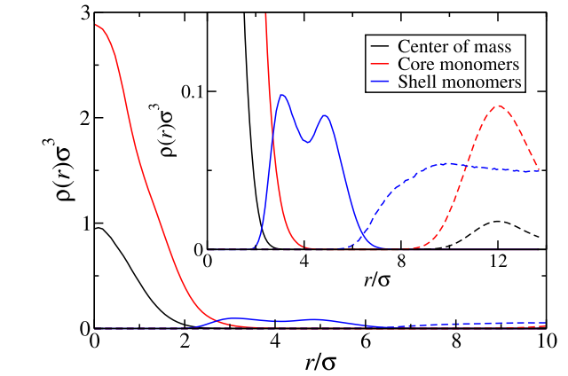
FIG. 11. Density profiles of the centers of mass, core, and shell monomers of Model II-dendrimers with respect to the center of mass of the cluster for a BCC crystal with \rho R_g^3 = 0.281 and N_{\text{occ}} = 8 . The solid curves represent contributions stemming from the same cluster, whereas the dashed curves in the inset are contributions from dendrimers belonging to different clusters.
