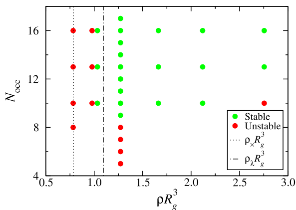
FIG. 6. The cluster size N_{\text{occ}} versus density \rho R_g^3 phase diagram of mechanical stability for FCC crystals of Model I. Stable systems are marked in green, unstable systems in red. The dotted and dashed-dotted lines are the densities for the predicted freezing and the Kirkwood instability, respectively.
