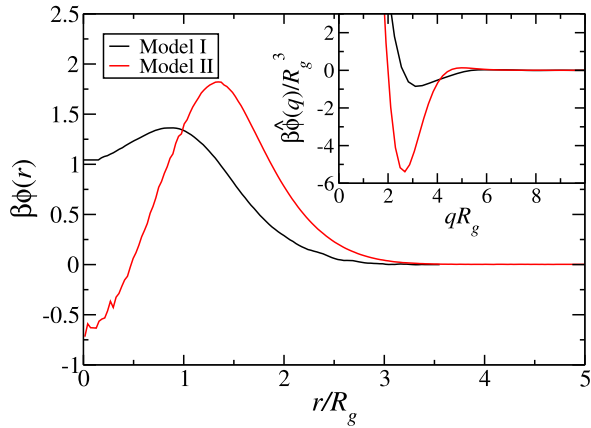
FIG. 2. The effective pair interaction \phi(r) between two amphiphilic dendrimers for both models. The inset shows the corresponding Fourier transforms \hat{\phi}(q) .
