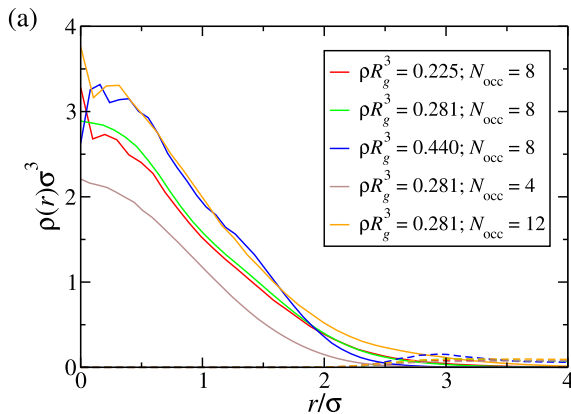
FIG. 12. Radial density profiles for all core and shell monomers with respect to the center of mass of the cluster in BCC crystals for various combinations of average cluster size and density. The solid curves and dashed curves correspond to profiles of core and shell monomers, respectively.
