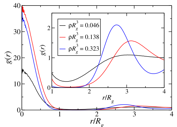
FIG. 3. The radial distribution function g(r) for the centers of mass of the dendrimers of Model II for three different densities, as indicated in the panel.
