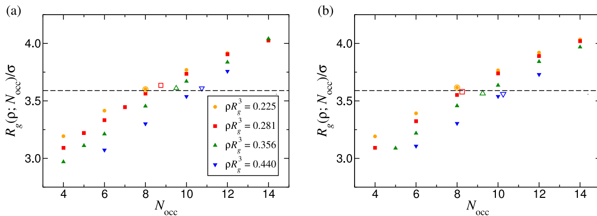
FIG. 8. The radius of gyration R_g(\rho; N_{\text{occ}}) of Model II dendrimers in (a) BCC and (b) FCC crystals. The open symbols denote the value for the thermodynamically stable crystals at the corresponding densities. The horizontal line indicates the value R_g = 3.58\sigma of the gyration radius of the dendrimers at infinite dilution.
