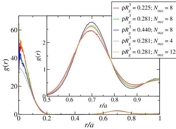
FIG. 10. Radial distribution function g(r) for the center of mass of Model II dendrimers in various FCC crystals, where the distance r is given in terms of the lattice constant a .
