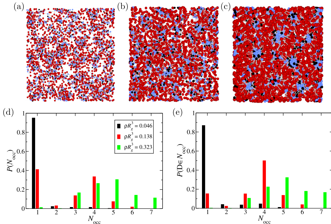
FIG. 4. Typical snapshots from the simulations of Model II systems at densities (a) \rho R_g^3 = 0.046 , (b) \rho R_g^3 = 0.138 , and (c) \rho R_g^3 = 0.323 , where the generation 0, 1, and 2 monomers (not drawn to scale) are shown in black, blue, and red, respectively. (d) presents the probability P(N_{\text{occ}}) of a cluster being formed by N_{\text{occ}} dendrimers. (e) shows the probability P(D \in N_{\text{occ}}) for a dendrimer to be found in a cluster of size N_{\text{occ}} .
