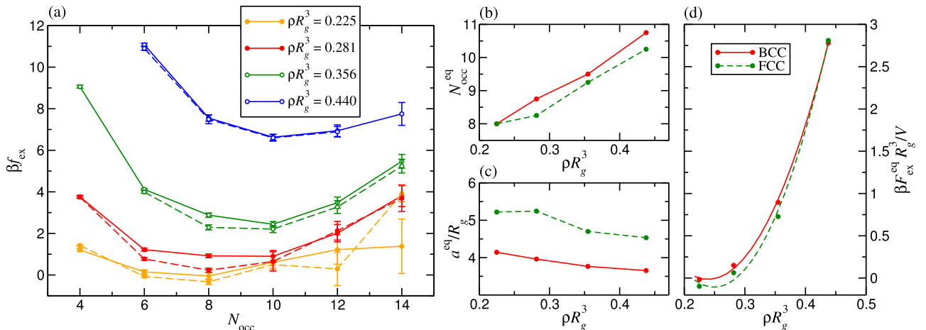
FIG. 14. (a) The excess free energy per particle, \beta f_{\text{ex}} , as a function of the cluster occupancy N_{\text{occ}} . The different colors correspond to constant overall densities. The equilibrium properties extracted are the (b) average cluster occupancy N_{\text{occ}}^{\text{eq}} , (c) lattice constant a , and (d) the excess free energy per volume \beta F_{\text{ex}}^{\text{eq}}/V as function of the overall density \rho R_g^3 . Solid and dashed lines correspond to BCC and FCC crystals, respectively.
